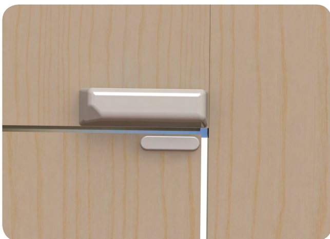
EMS mounted on door frame with magnet
