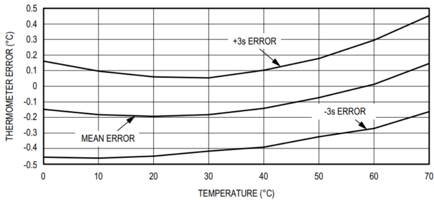
DS18B20 TYPICAL ERROR CURVE
